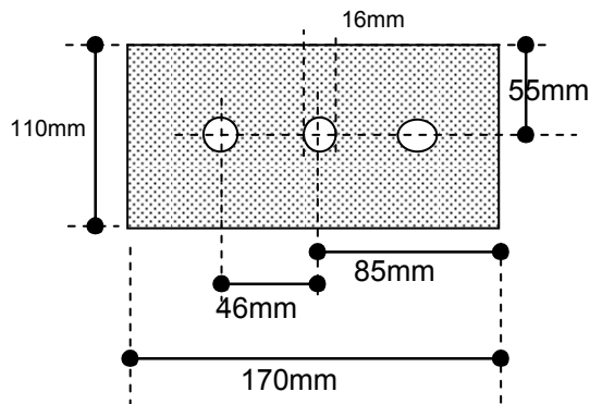
CABLE ENTRY COVER PLATE
