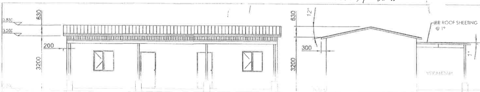
FRONT ELEVATION SCALE 1:100
