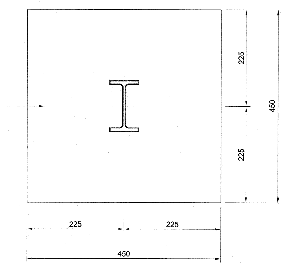
SECTIONAL PLAN B-B TYPE "A1" 1:5
