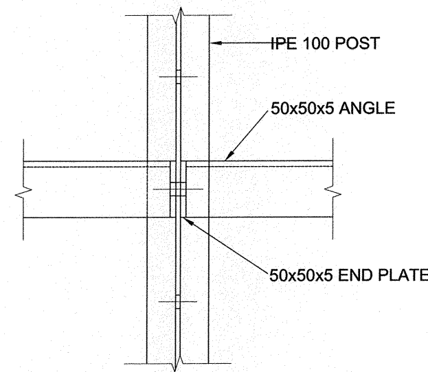
DETAIL 1 TYPICAL CONNECTION DETAIL 1:5
