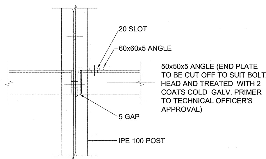
DETAIL 2 TYPICAL EXPANSION JOINT DETAIL 1:5
