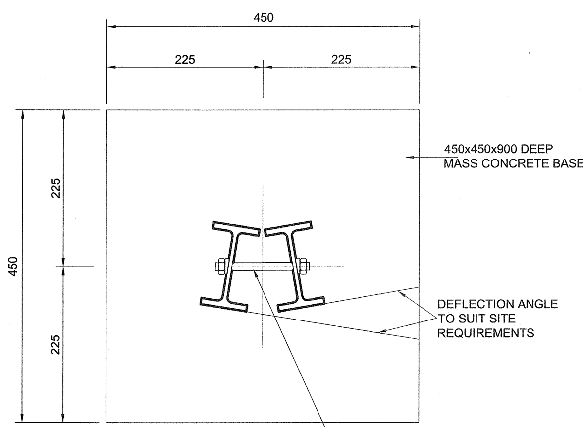
DETAIL OF MASS CONCRETE BASE WITH CHANGE OF DIRECTION TYPE "A2" 1:5
