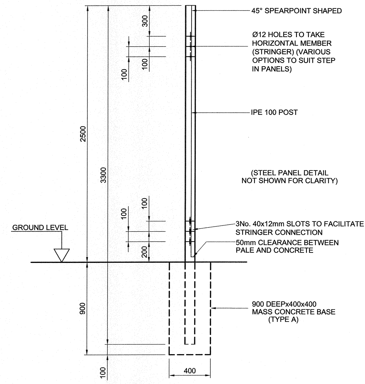
TYPICAL SECTION A-A 1:20
