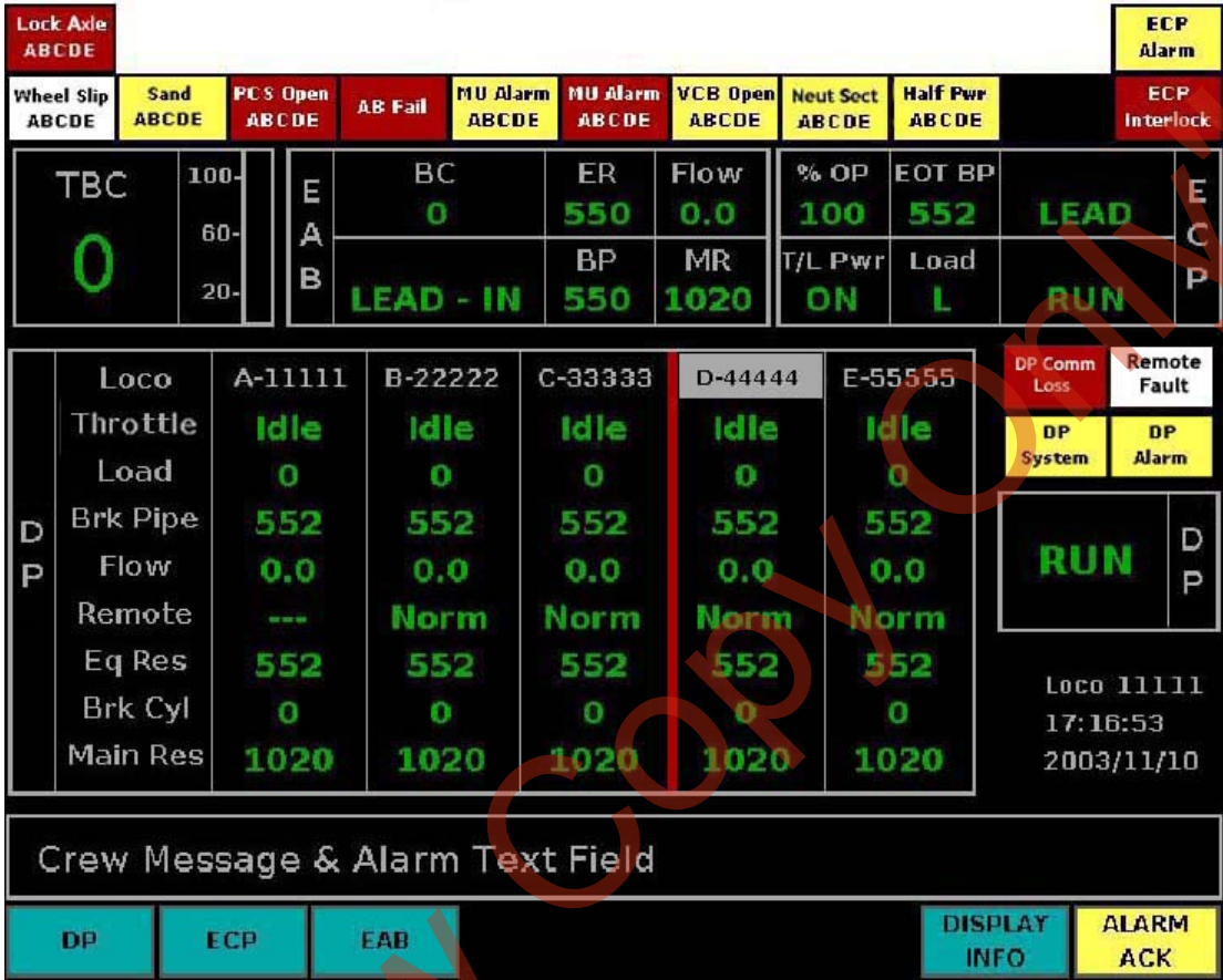
Figure 3: Wired Distributed Power (WDP)
